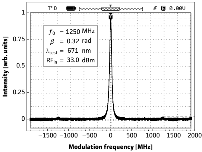
Fig. 1: Oscilloscope trace
